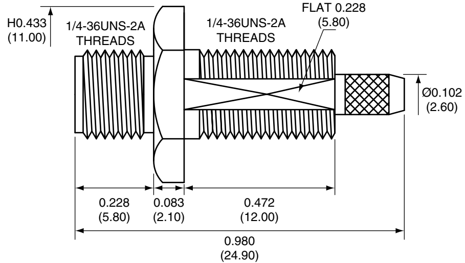
SIDE VIEW
